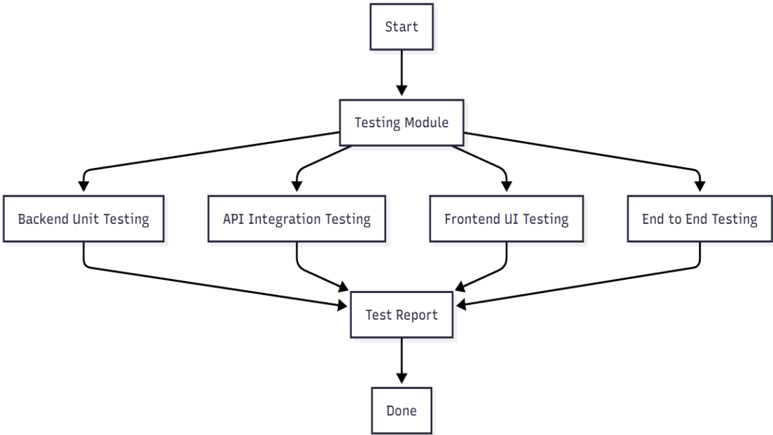
Figure 5.6.2: Testing Sequence Digram
